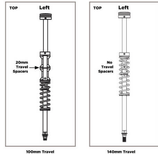
Example: Changing the 140mm travel fork into a 100mm travel fork using travel spacer.
