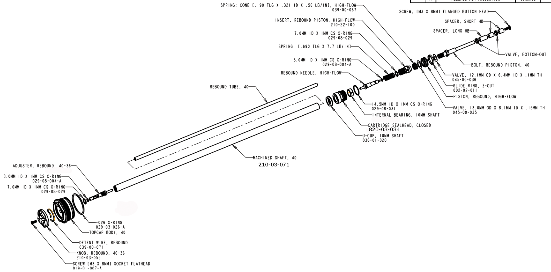
Top Cap Assembly: 820-05-020
